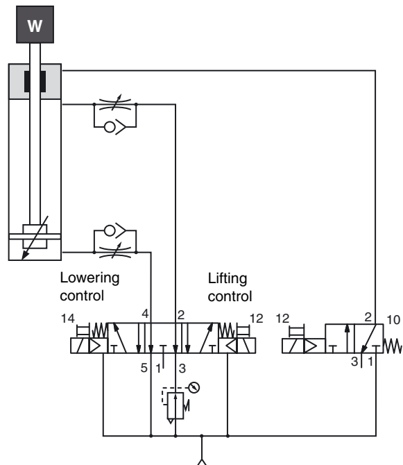
Fig. 4 - Load on top of the cylinder
